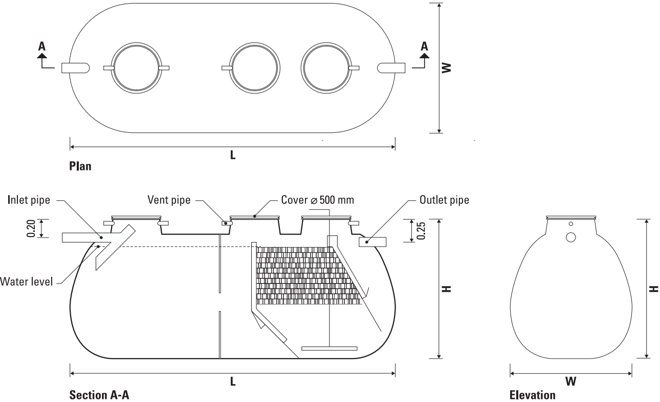
Tank schematic
