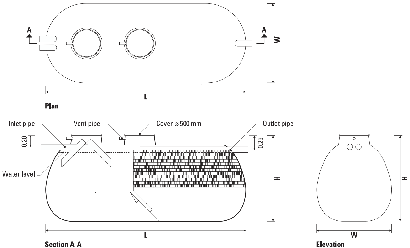
Tank schematic
