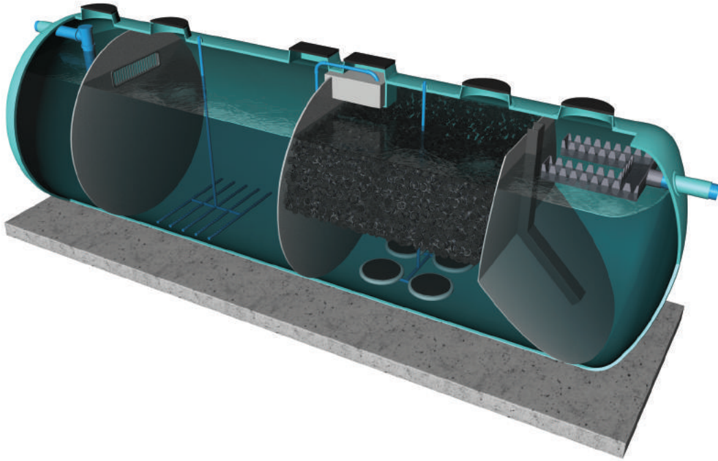
Tank schematic
