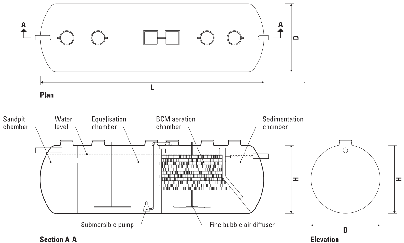
Tank schematic
