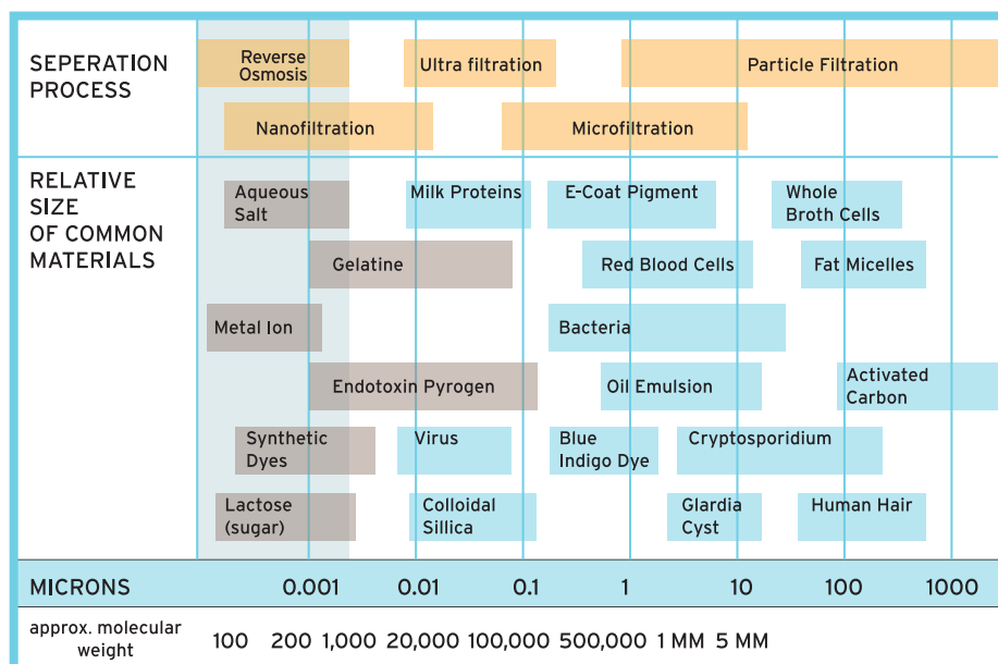
MEMBRANE FILTRATION SPECTRUM
