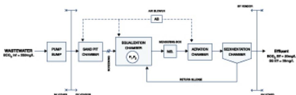
WASTEWATER TREATMENT FLOW DIAGRAM
